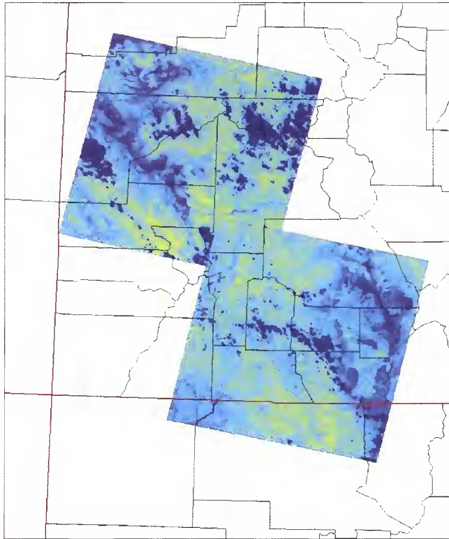
Figure 4. Logistic regression model of HPS risk in southern Colorado and north-central New Mexico. State boundaries (red lines) and county boundaries (black lines) are indicated for relationship to the study area shown in Figure 1. Risk is shown in 2005 (A) and 2006 (B), using Landsat TM imagery from 2004 and 2005, respectively. Risk in 2005 (A) was generally low, except for several diffuse areas of moderate–high risk in Colorado. In 2006 (B), HPS risk appears to be markedly increased in extent and intensity throughout much of the region. The color scale is as shown for Figure 1.
